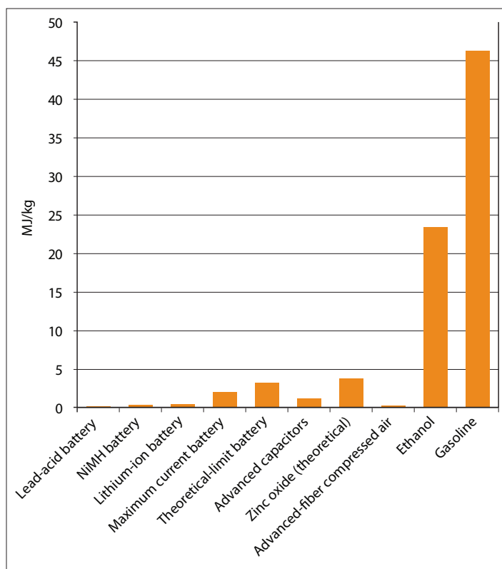
FIGURE 18.1 Comparison of energy densities.
